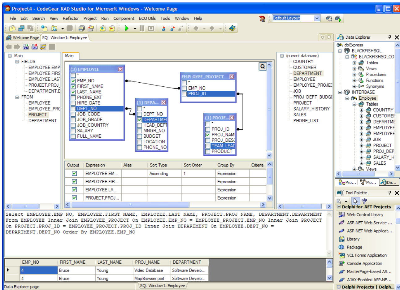
Figure 17. SQL Window
