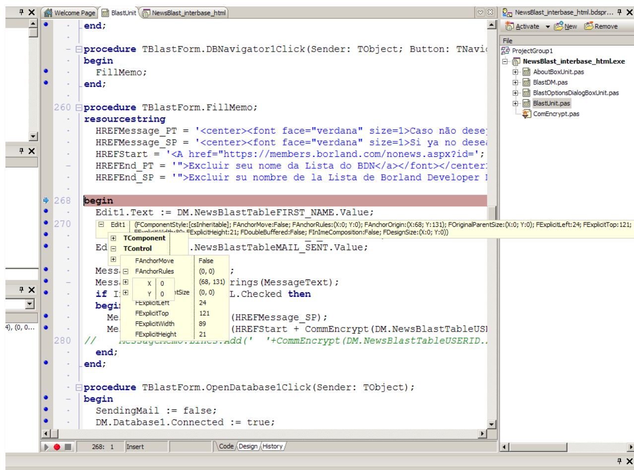
Figure 19. Debugger
